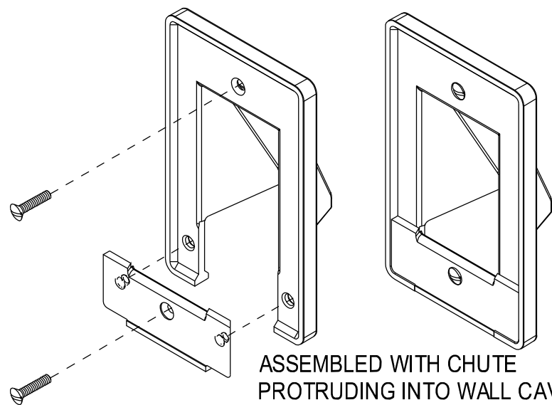
ISOMETRIC VIEWS
