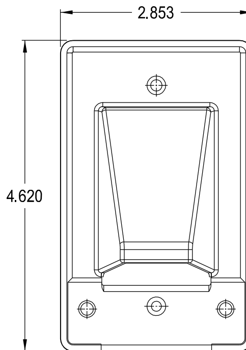
ASSEMBLED WITH CHUTE PROTRUDING FROM WALL
