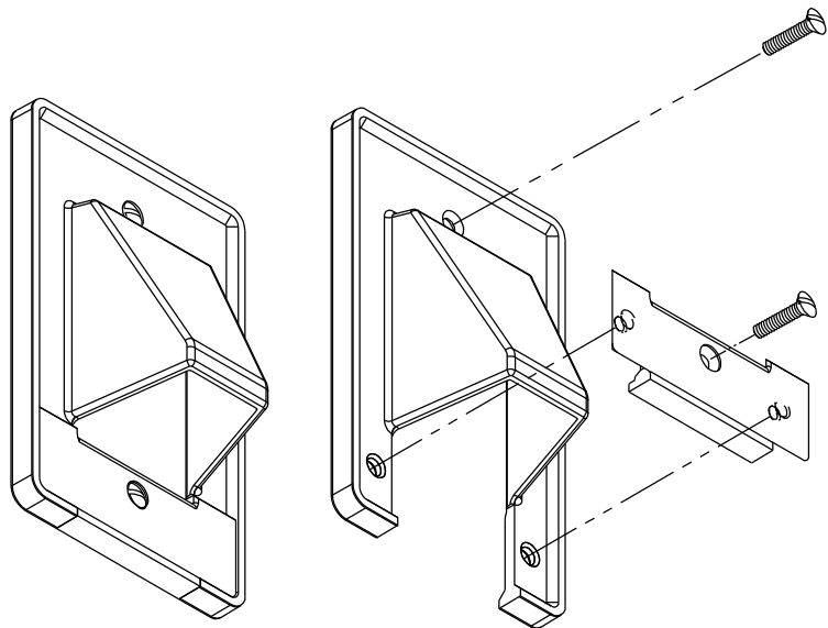
ASSEMBLED WITH CHUTE PROTRUDING FROM WALL
